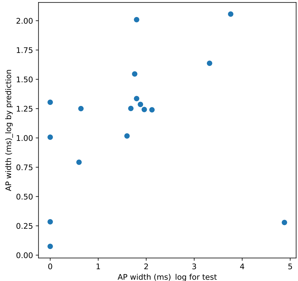
prediction of AP width (ms)_log by embs alpha 0.30000000000000004 l1_ratio 0.05 MAE 0.915
